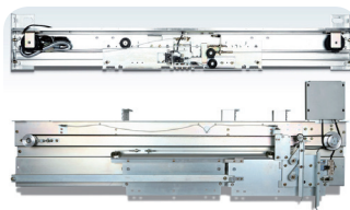
Landing Door Operator
